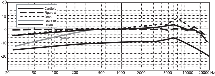
C03U FREQUENCY RESPONSE
