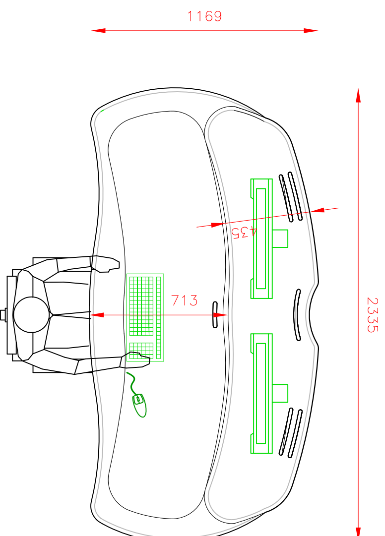
PLAN VIEW
