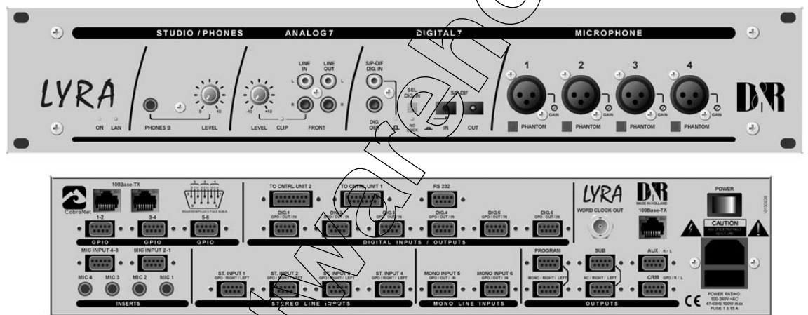
I/O RACK FRONT AND BACK VIEW
