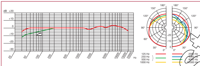
Frequency response and polar pattern
